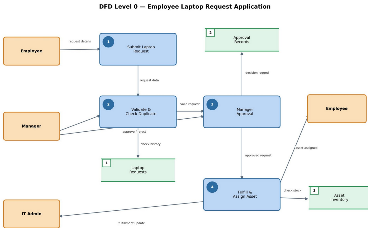
Figure 1 — DFD Level 0 — Employee Laptop Request Application
